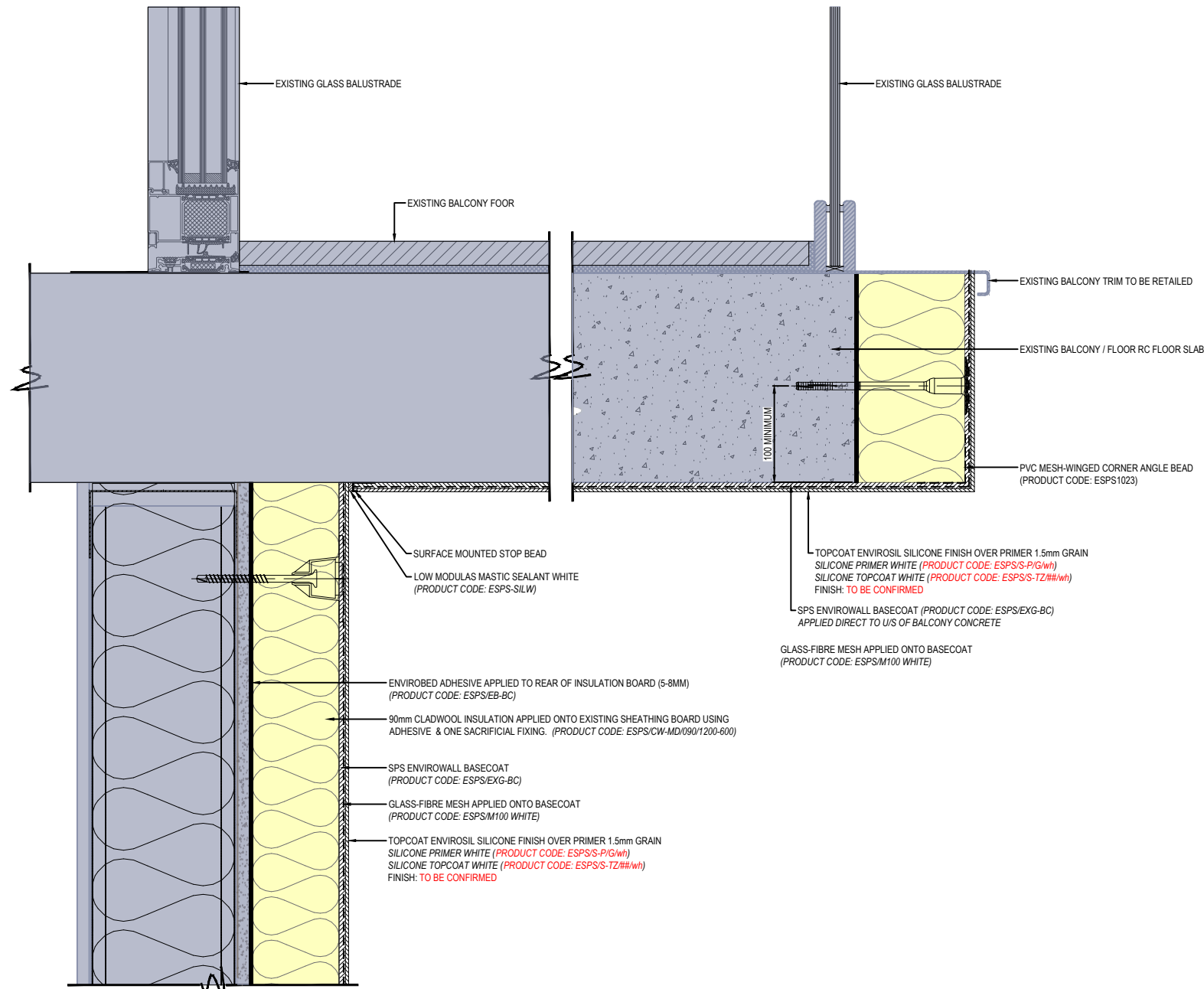
03 CROSS SECTION - RENDER / RECESSED BALCONY Scale 1:3
