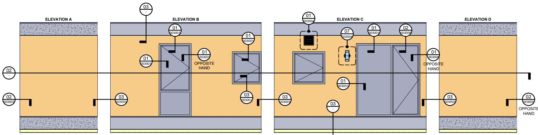
01 UNROLLED ELEVATIONS - RENDER / RECESSED BALCONY Scale 1:35
